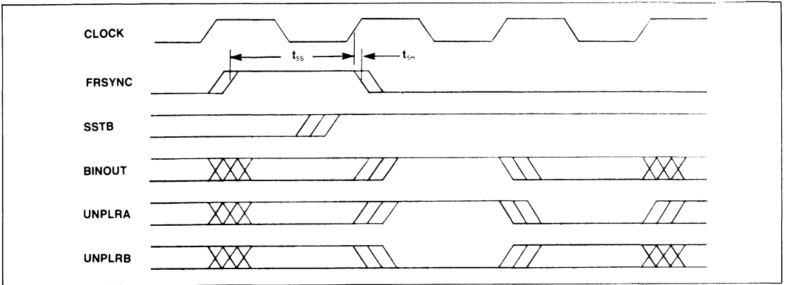
Figure 6. Non-return-to-zero FRSYNC Timing
