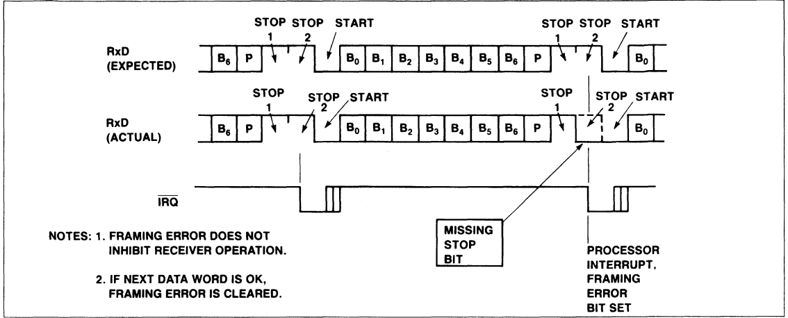
Figure 12. Framing Error
