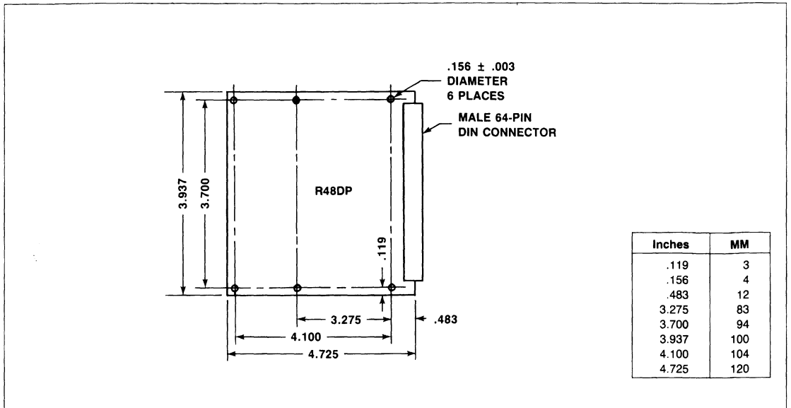
R48DP Circuit Board Dimensions
