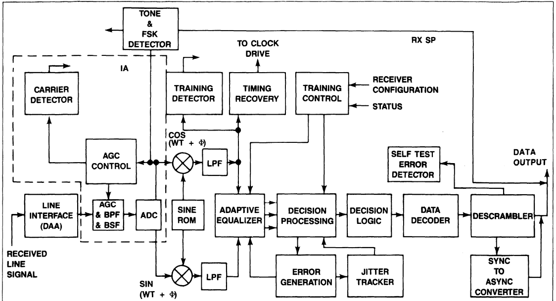
R1212 Receiver/Equalizer Block Diagram
