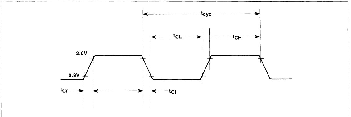
Figure 44. Input Clock Waveform
