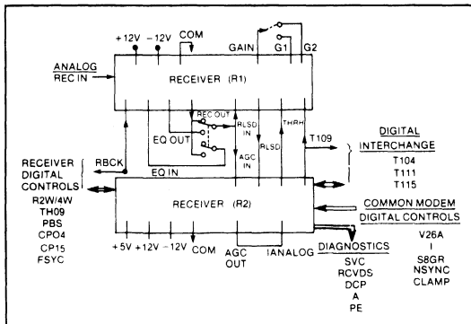
Figure 2. Receiver Interconnection
