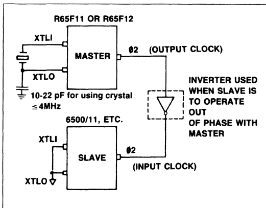
Figure 3-4. Master/Slave Connections
