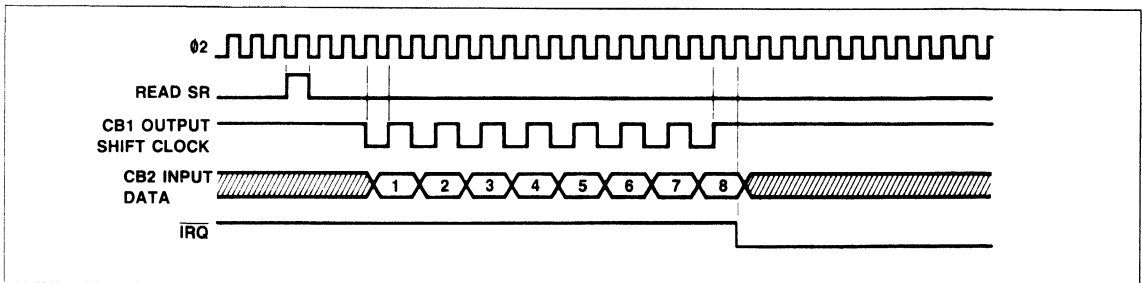
Figure 23. SR Mode 2 — Shift In Center Ø2 Control
