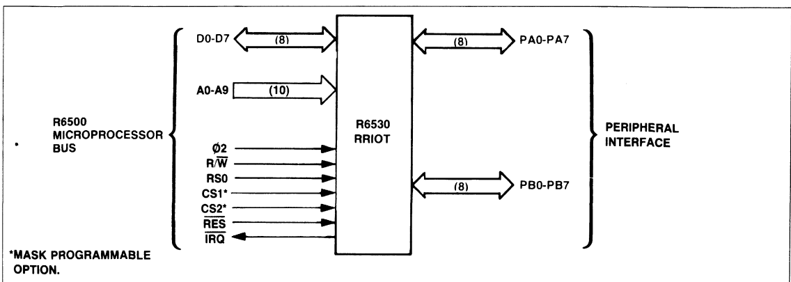
Interface Signals
