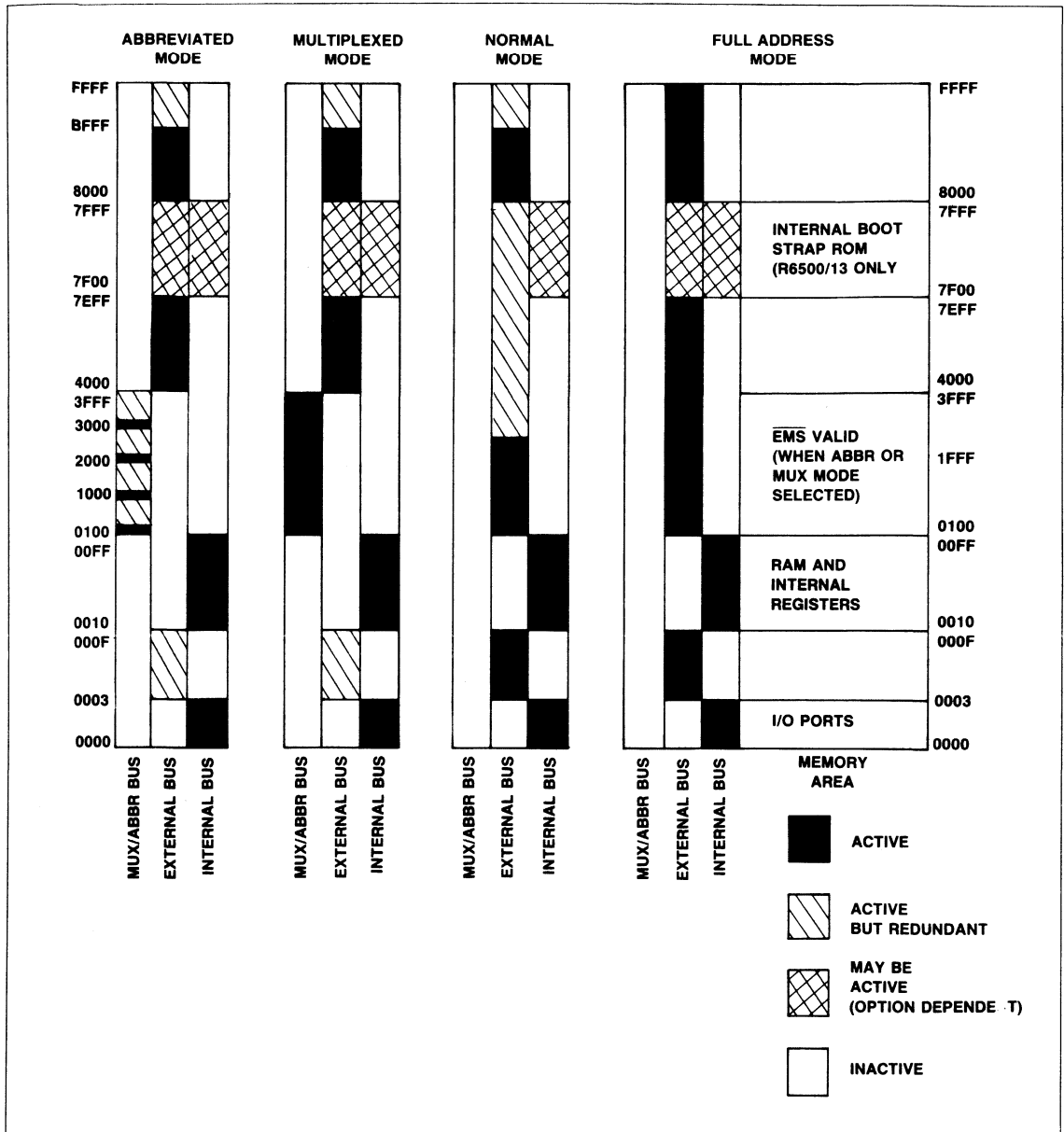
Figure 4-2. Memory Map
