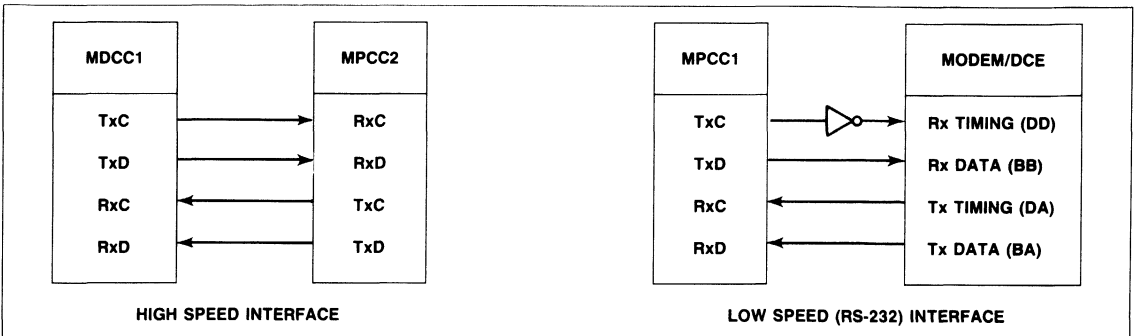
Figure 18. Serial Interface
