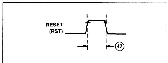
Figure 18. Reset Timing
