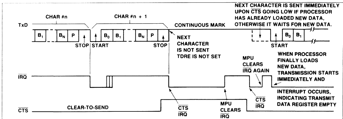
Figure 9. Effects of \overline{\text{CTS}} on Transmitter
