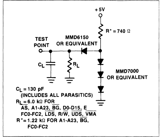
Figure 43. Test Loads
