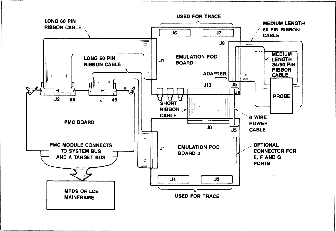
System Interconnection
