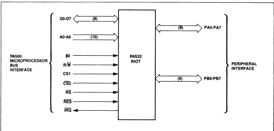
RIOT Interface Signals
