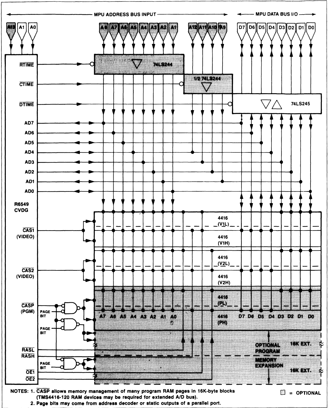
Figure 6. CVDG Connection to A/D Bus and DRAM
