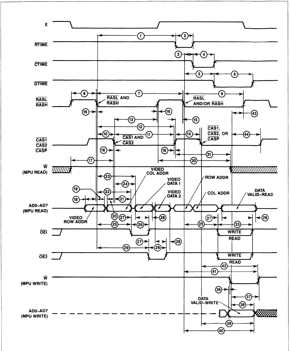
Figure 9. CVDG-DRAM A/D Bus Timing Waveforms
