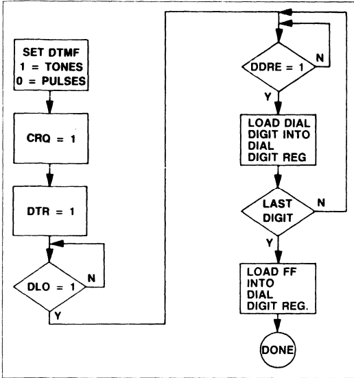
Auto Dial Sequence Flow Diagram
