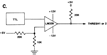
Suggested Interface Circuits for Controlling THRESH1 and THRESH2 Input Lines
