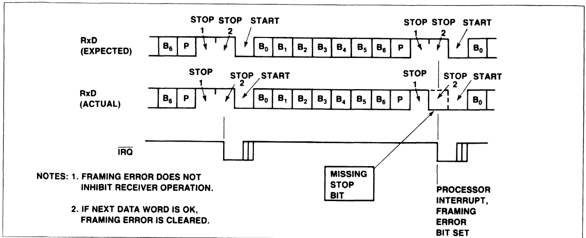
Figure 12. Framing Error
