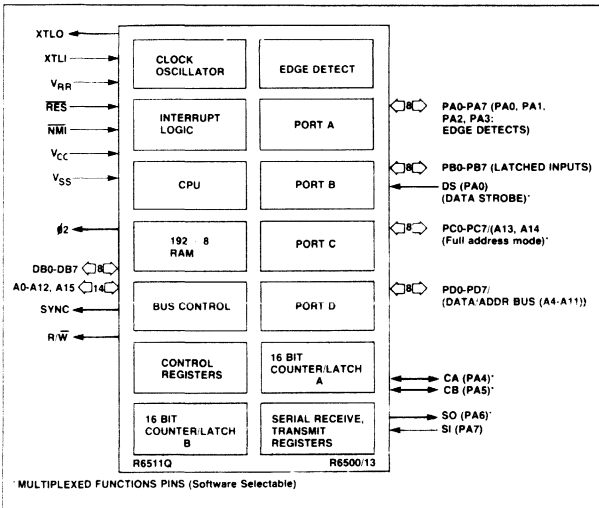
Figure 2-2. Interface Diagram
