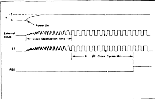
Figure 7-1. Power Turn-On Timing Detail
