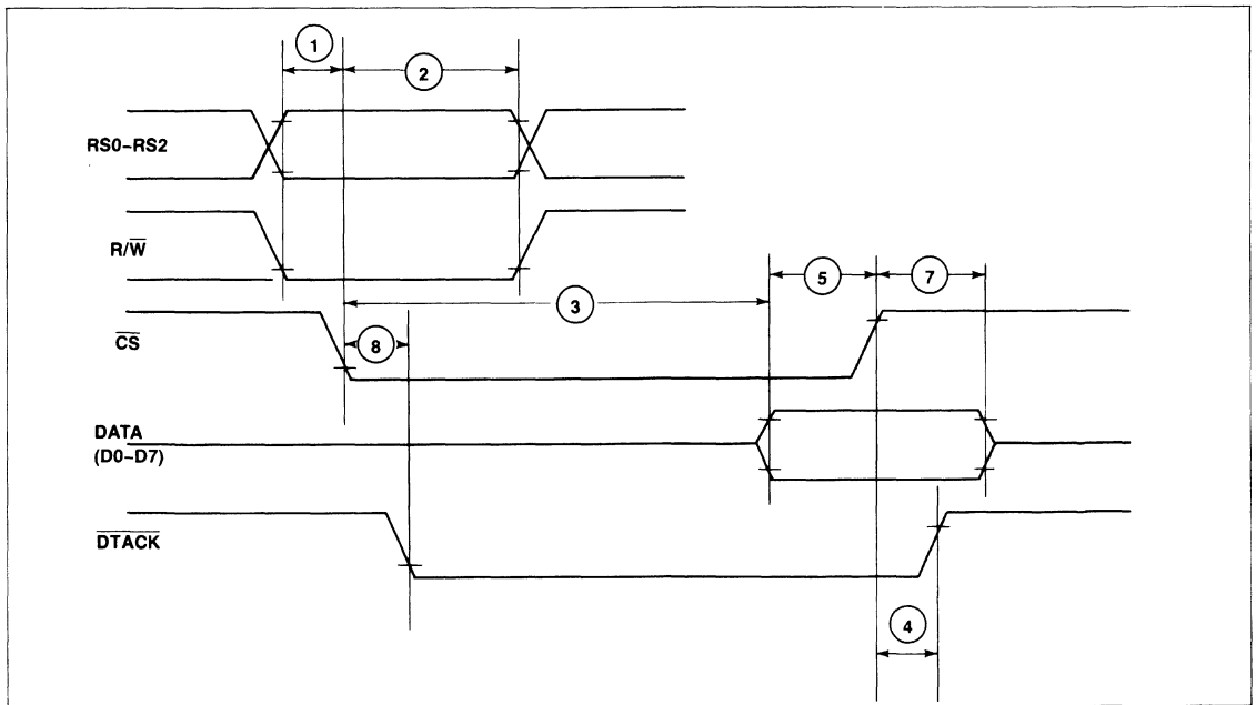
DACIA Write Cycle Timing
