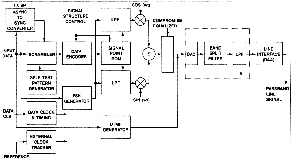
R1212U Transmitter Block Diagram
