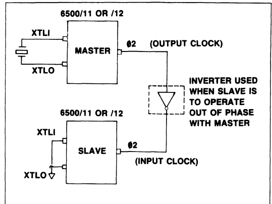
Figure 3-4. Master/Slave Connections
