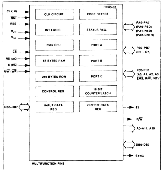
Figure 2-1. Interface Diagram
