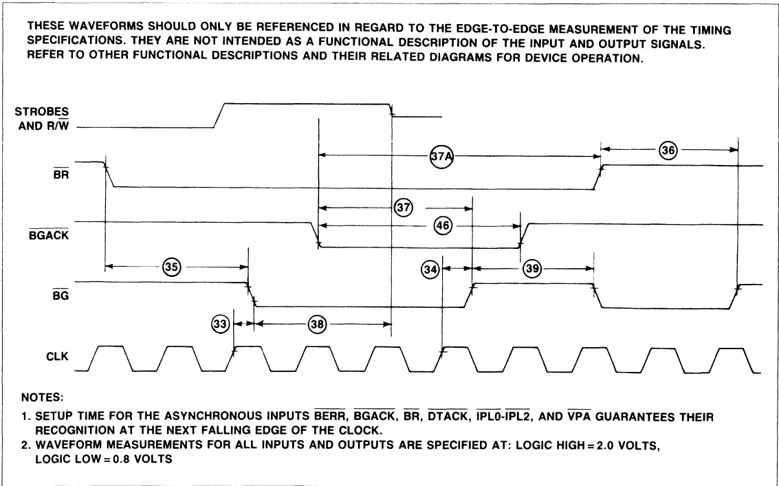
Figure 47. AC ELECTRICAL Waveforms — Bus Arbitration
