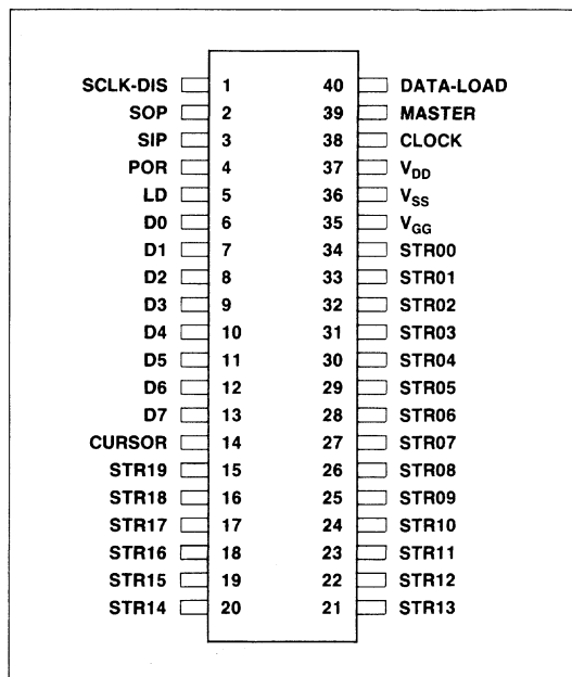
10939 Pin Configurations
