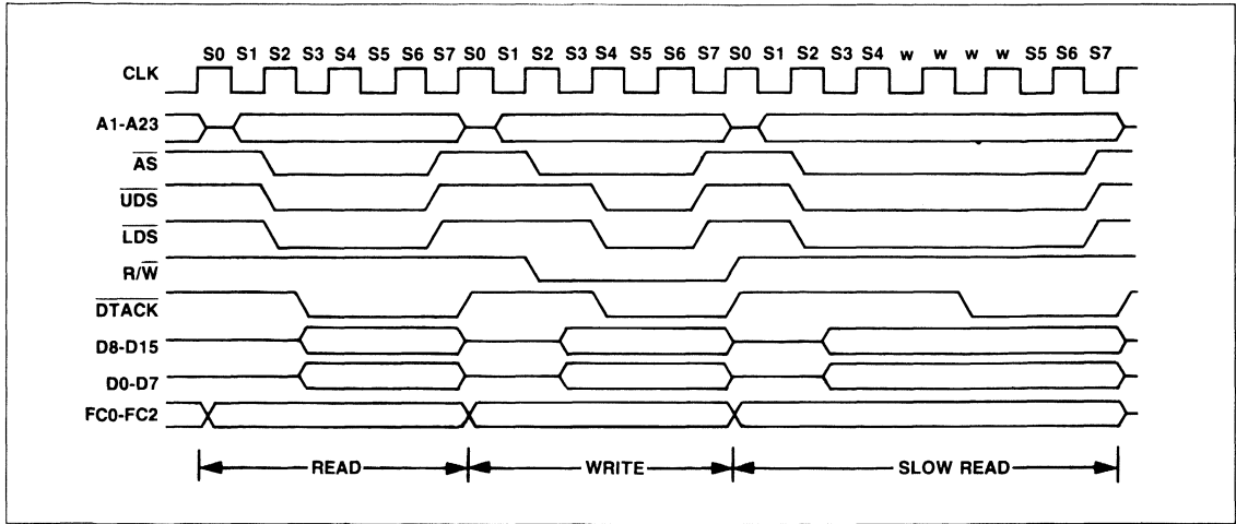
Figure 6. Read and Write Cycle Timing Diagram
