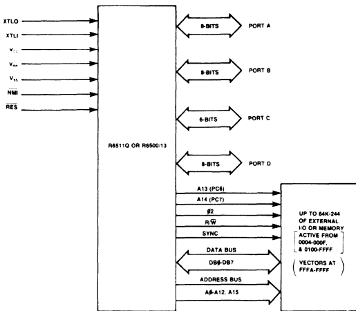
Figure 4-1a. Full Address Mode
