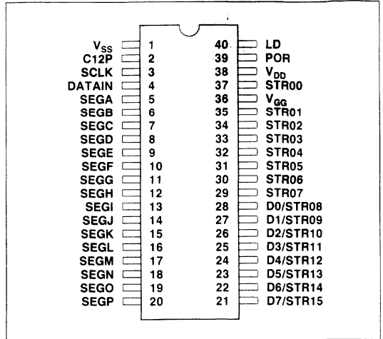
10955 Pin Configuration
