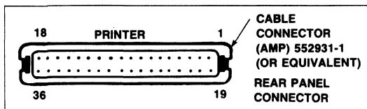
External Printer Connector
