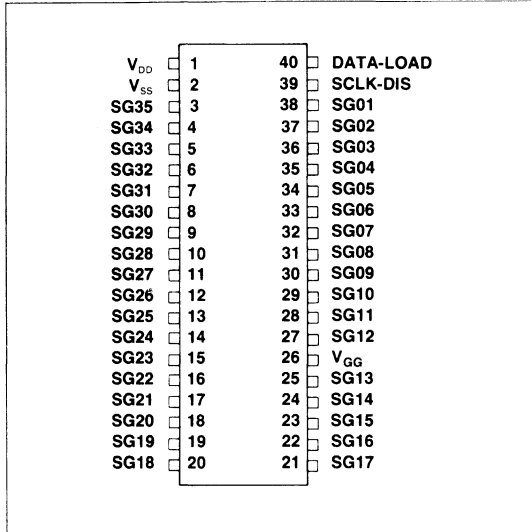
10938 Pin Configuration
