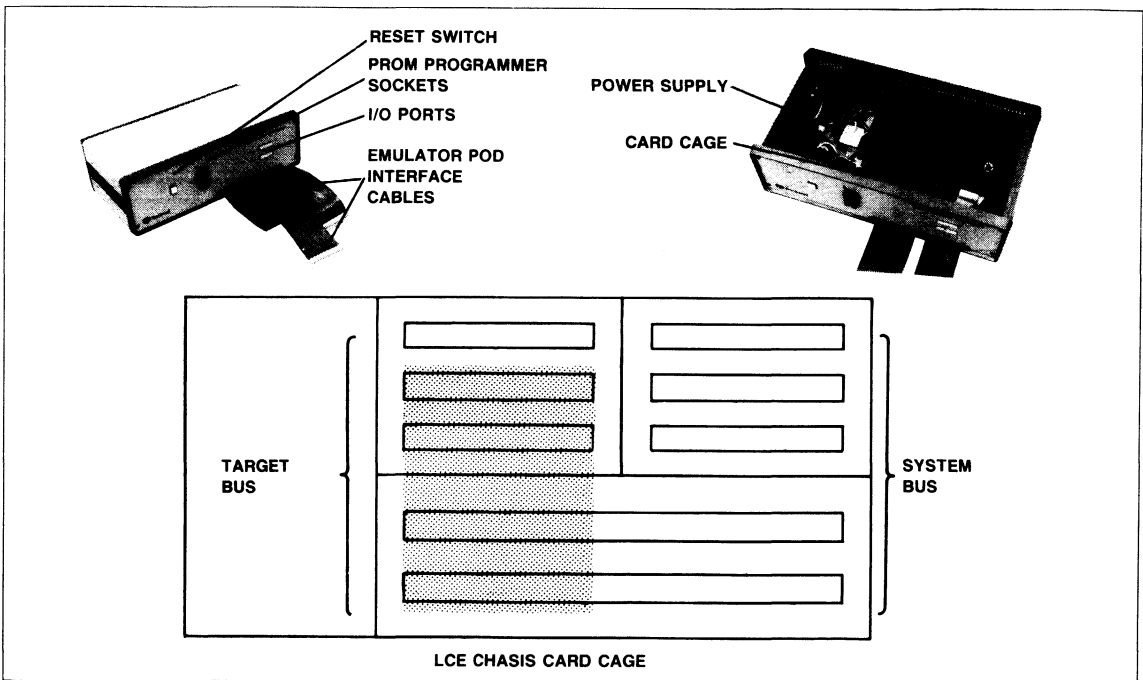
LCE Internal Layout and Card Cage Bus Structure
