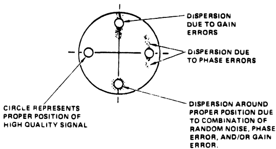
Typical Eye Pattern: 4 Phase-2400 BPS-1200 Baud (V26A)
