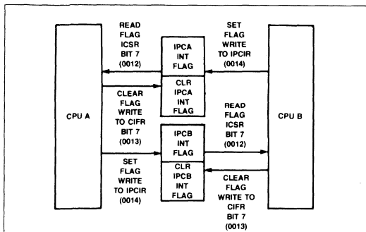
Figure 7. Inter Processor Communication
