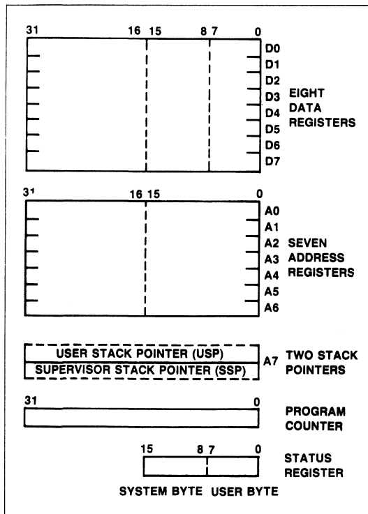
R68000 Registers
