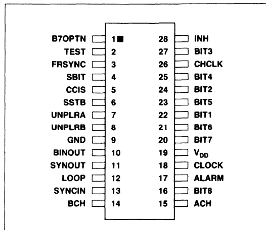
Pin Configuration
