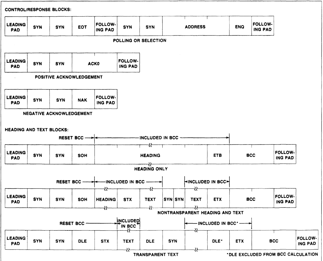
Figure 8. BSC Message Format Examples
