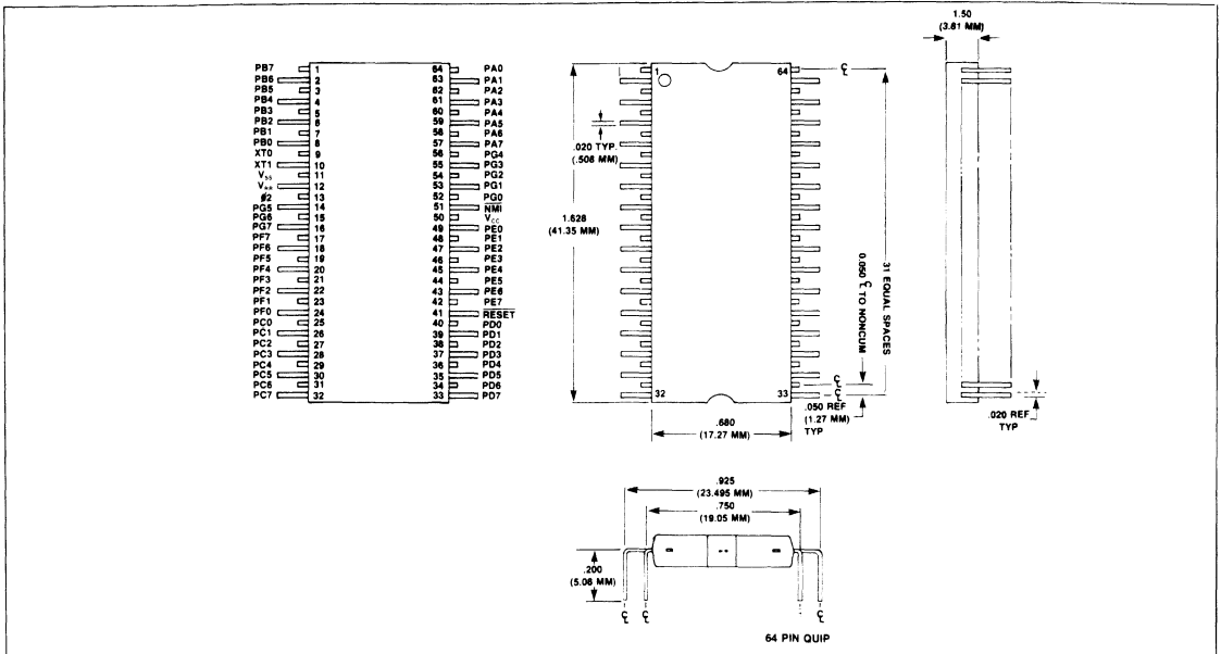
Figure 2-3. R6500/12 or /16 Mechanical Outline and Pin Out Configuration
