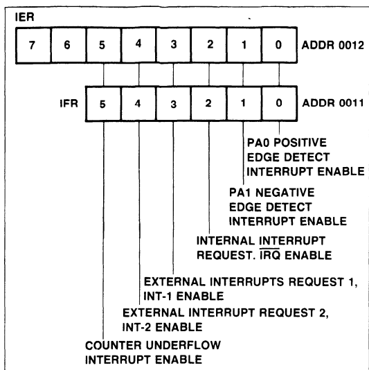
Figure 3-3. Interrupt Enable and Flat Registers
