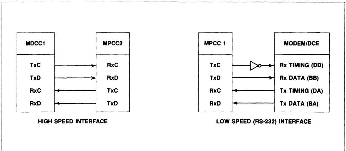
Figure 17. Serial Interface
