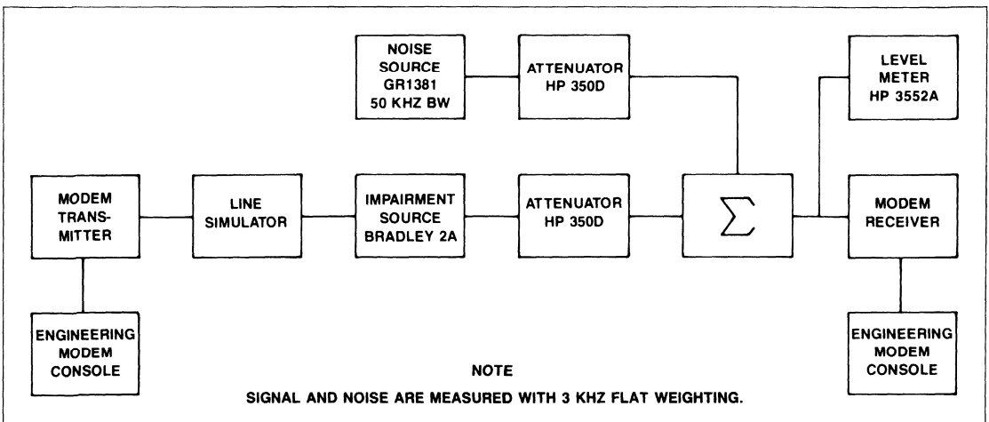
BER Performance Test Set-up
