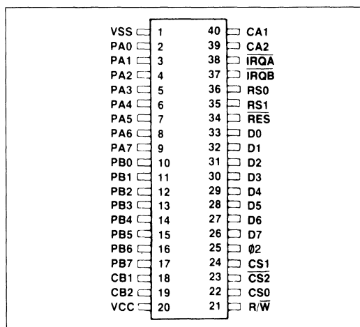
Figure 1. R65C21 Pin Configuration
