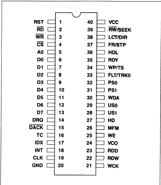
DDFDC Pin Diagram
