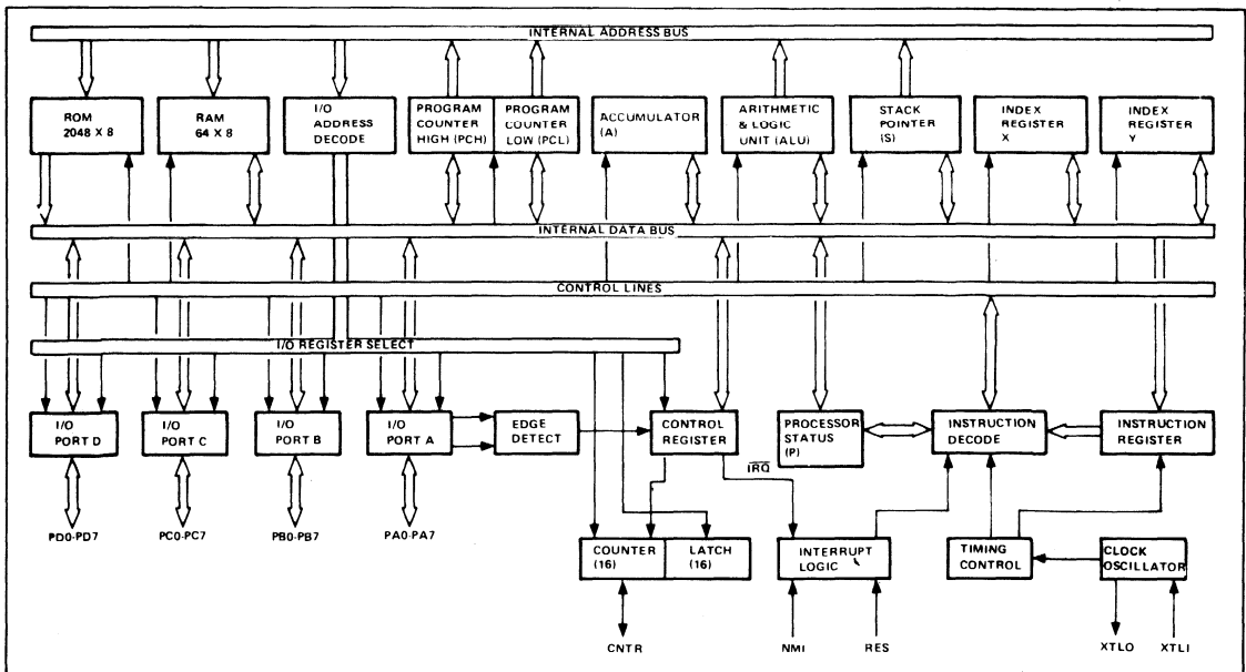
Figure 3-1. R6500/1 Block Diagram
