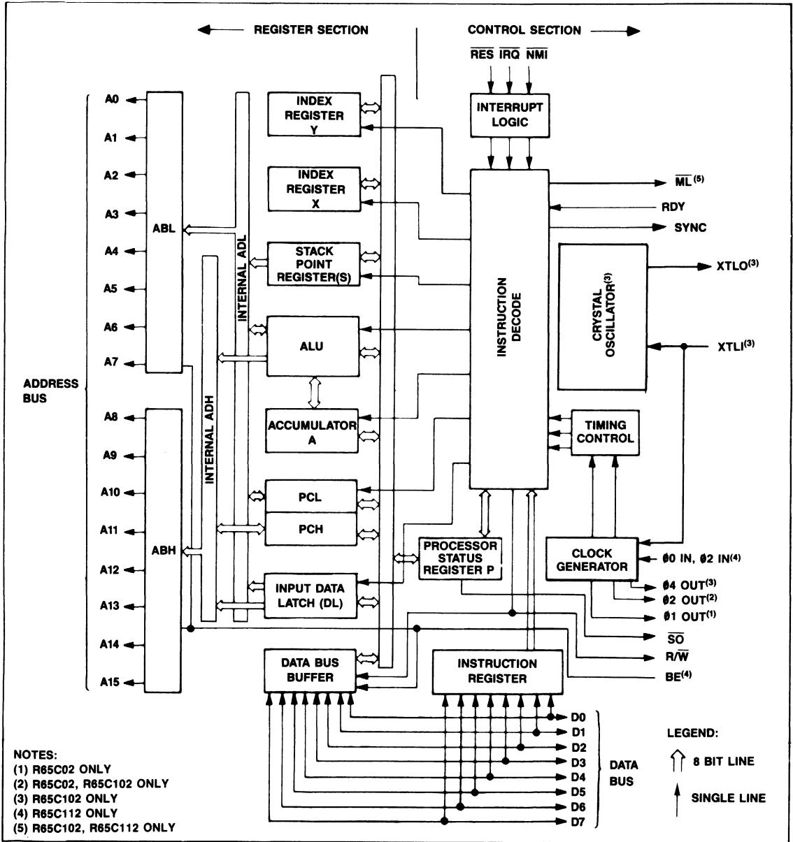
Figure 1. R65C00 Internal Architecture
