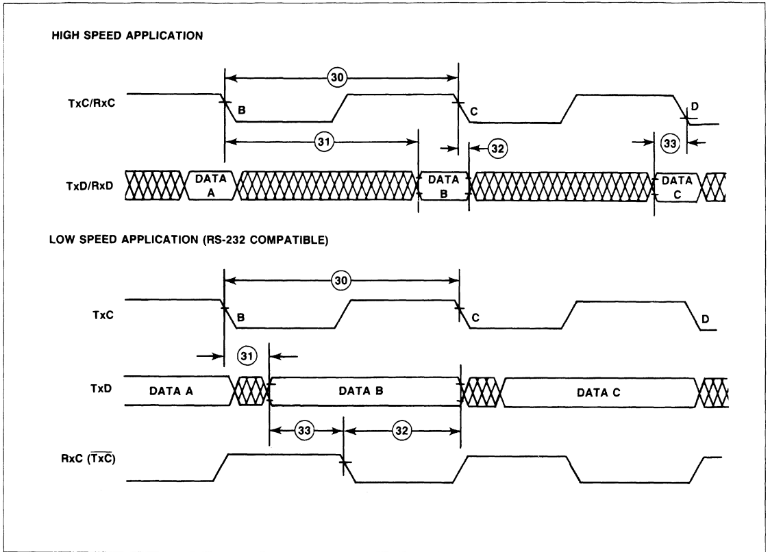
Figure 18. Serial Interface Timing
