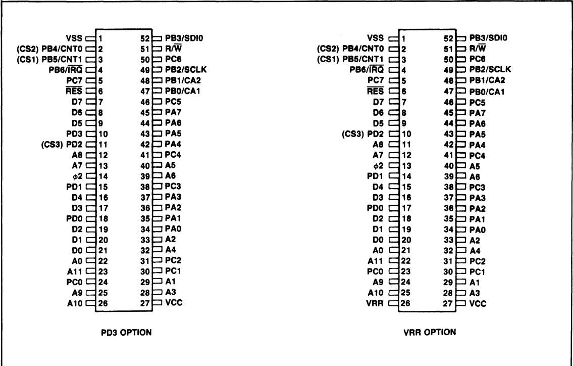
R6531Q 52-Pin QUIP Configurations
