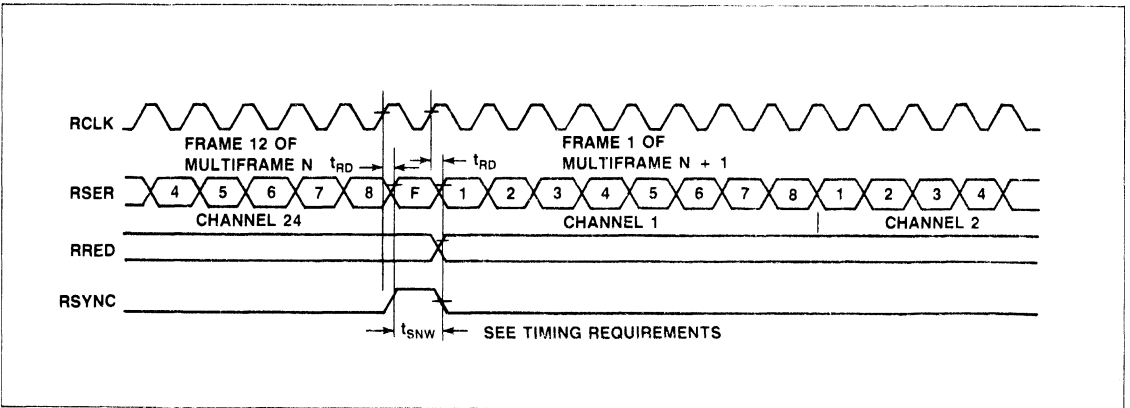
North American 193 Mode Receive Synchronization Timing
