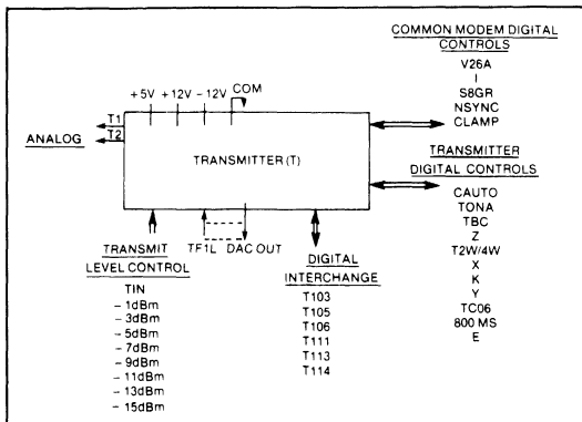
Figure 1. Transmitter Interfaces
