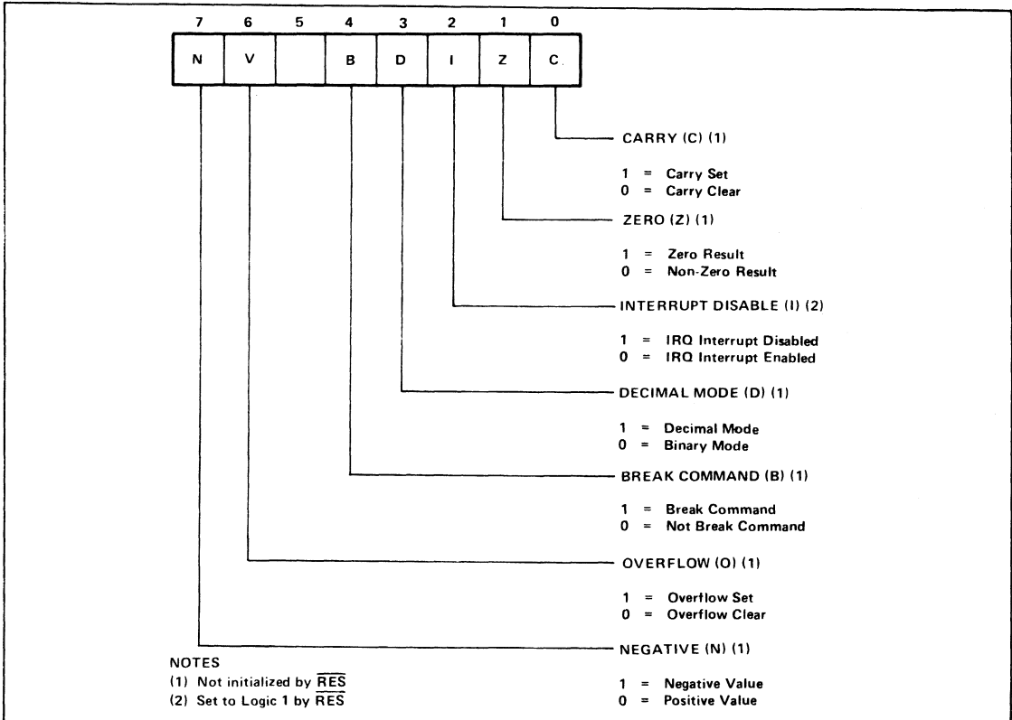
Figure 3-3. Processor Status Register
