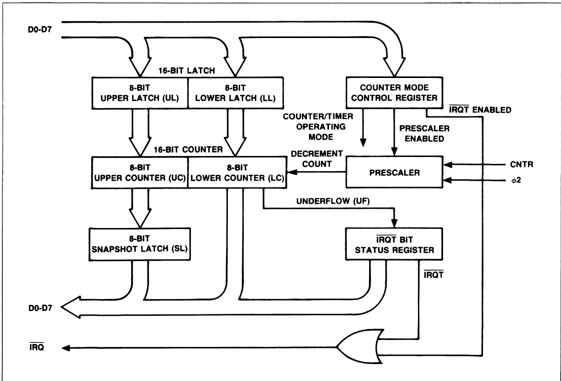
Figure 3. Counter/Timer
