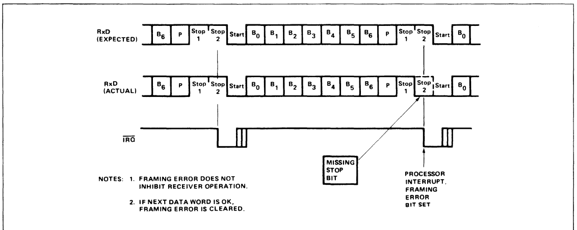
Figure 13. Framing Error
