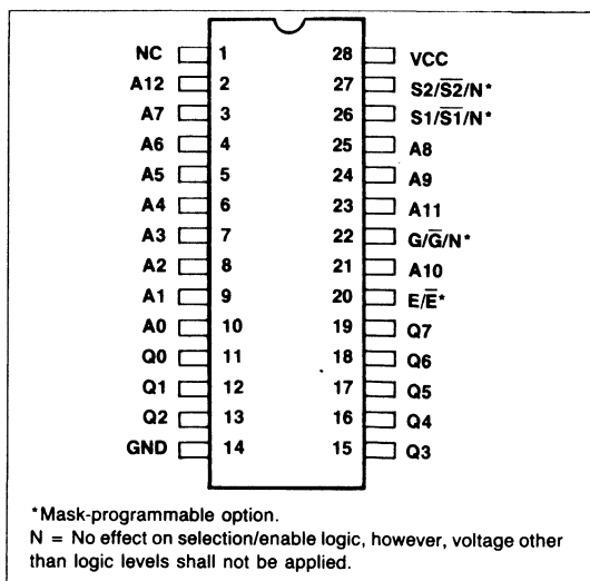
R2364B Pin Configuration
