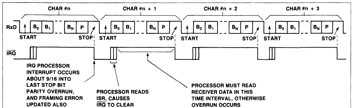
Figure 7. Continuous Data Receive
