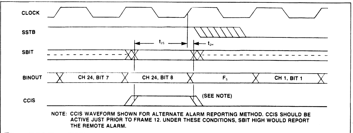
Figure 4 (c). Control Input Timing
