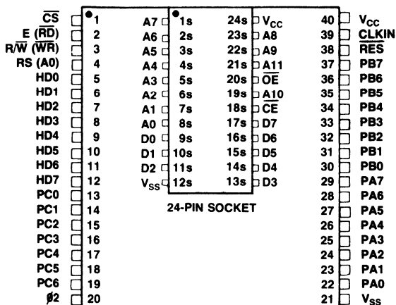
Pin Configuration
