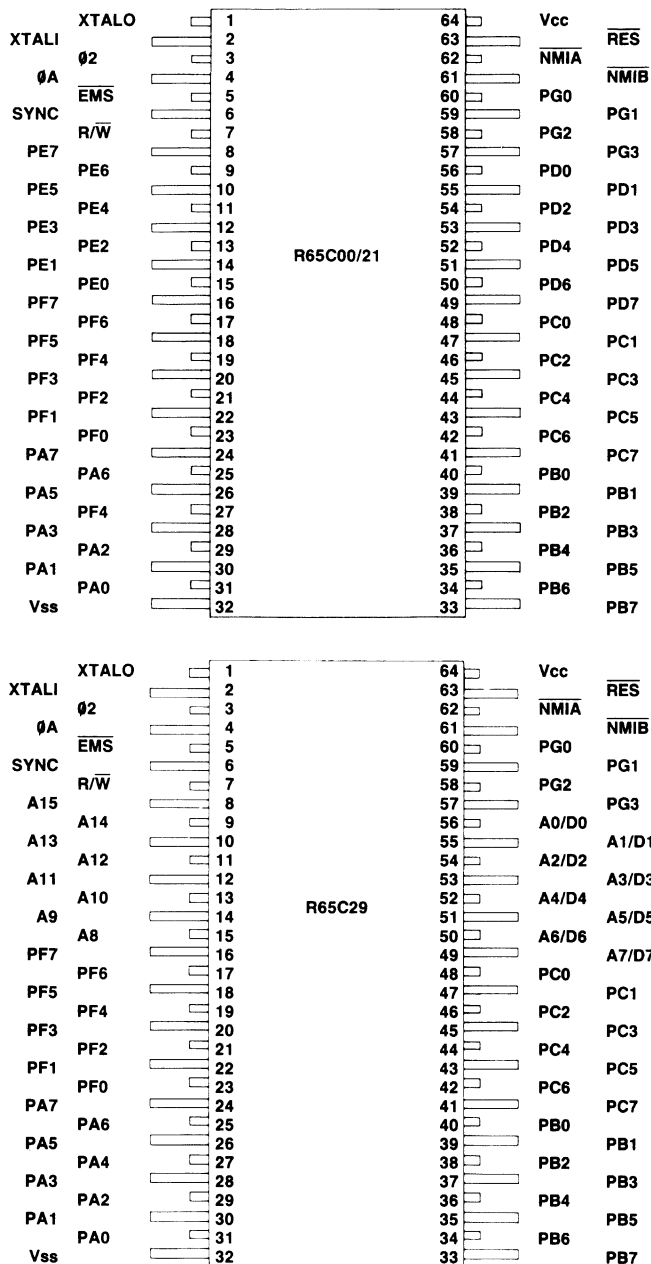
Figure 2. R65C00/21 and R65C29 Pin Assignments
