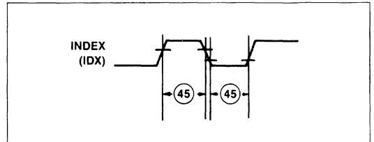
Figure 16. Index Timing
