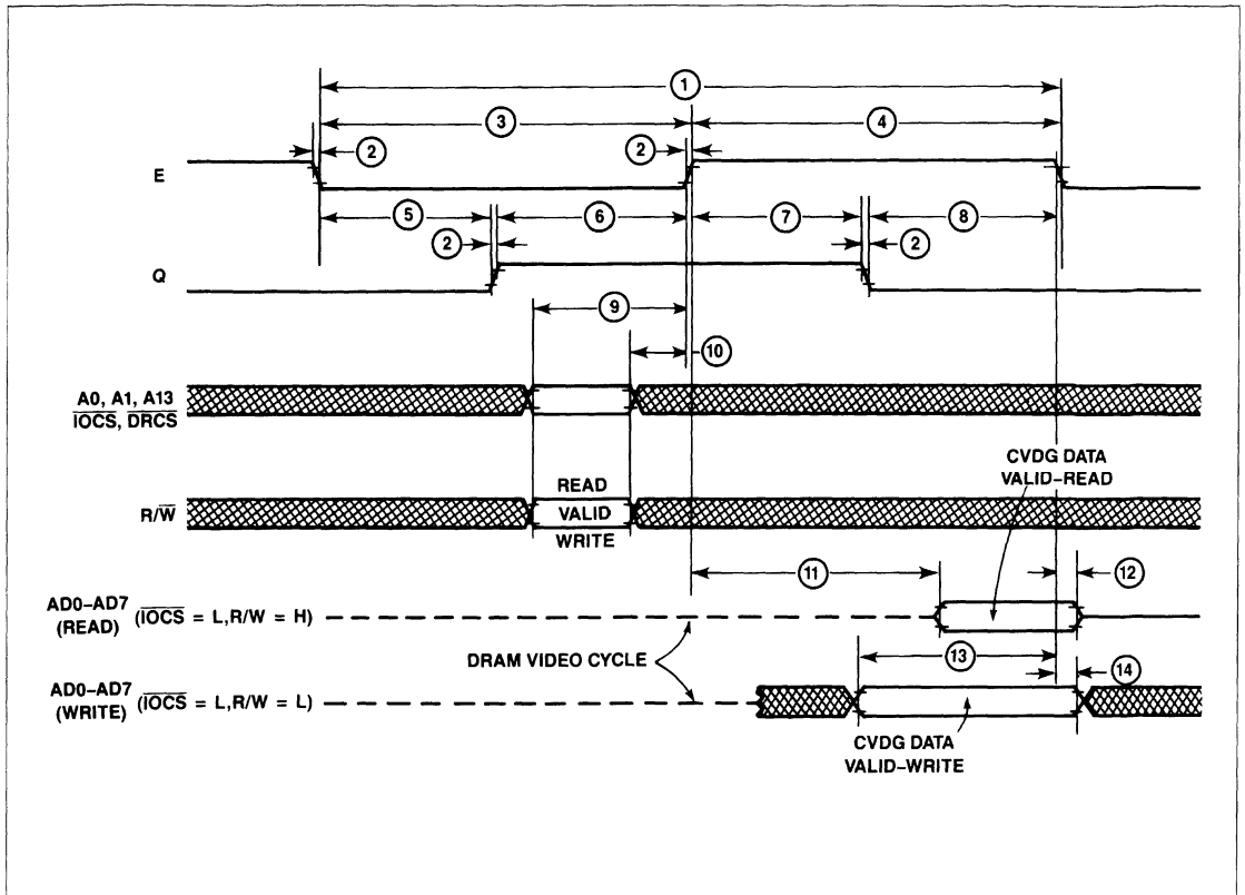
Figure 8. CVDG-MPU A/D Bus Timing Waveforms
