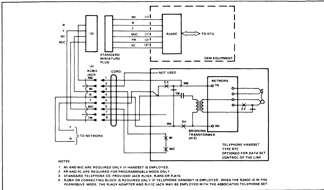
Typical R24DC to Network Interconnection
