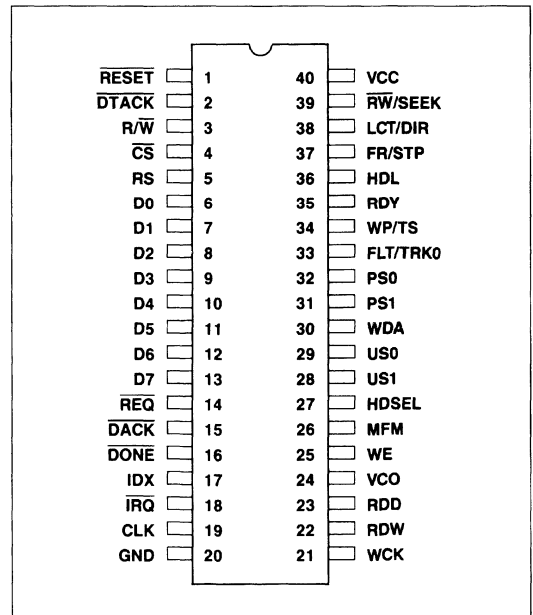
Pin Diagram
