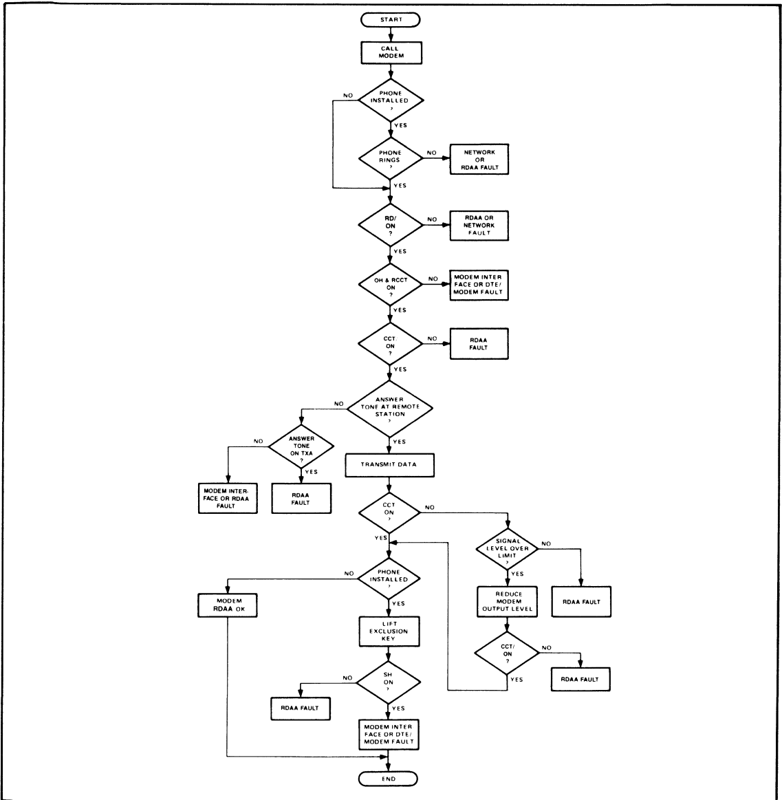
Figure 9. RDAA Fault Isolation Flow Chart
