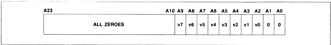
Figure 26. Address Translated From 8-Bit Vector Number
