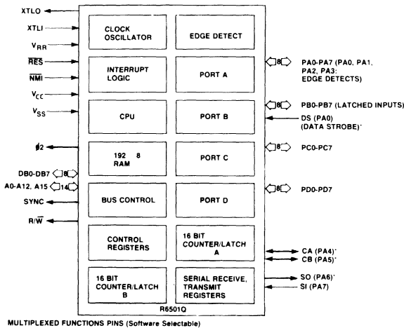
Figure 2-2. Interface Diagram
