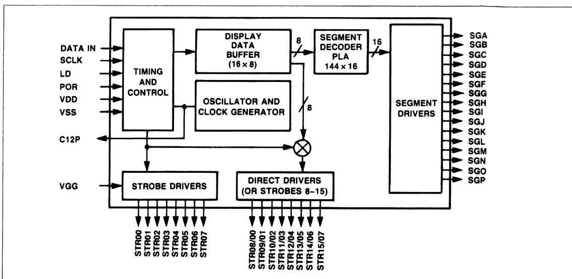
10955 Block Diagram
