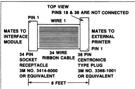
Printer Interface Cable (User Supplied)
