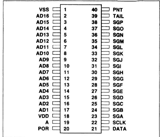
Pin Configuration
