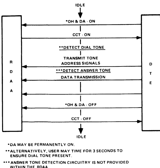
Figure 8. Touch-Tone Origination Sequence
