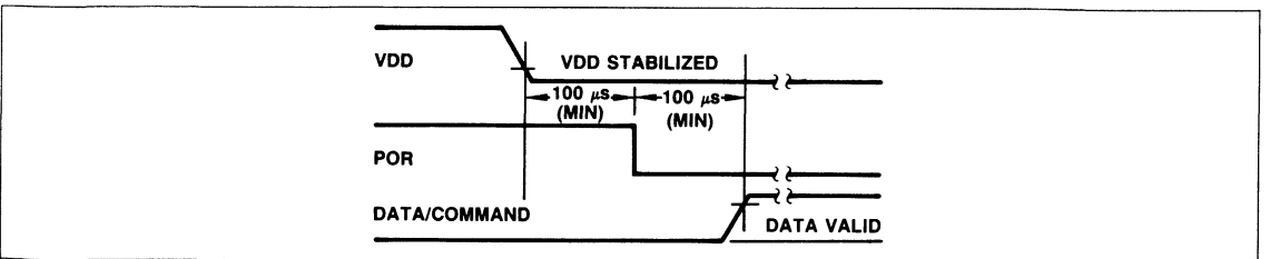
Power-On Reset
