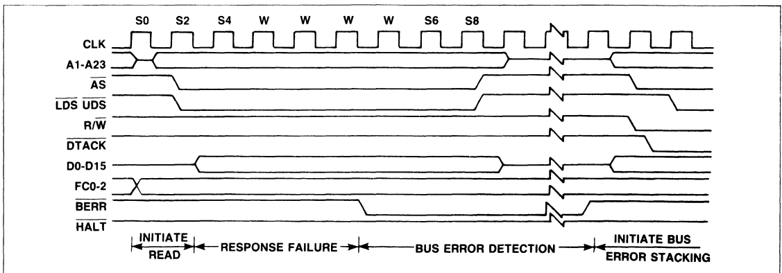
Figure 20. Bus Error Timing Diagram
