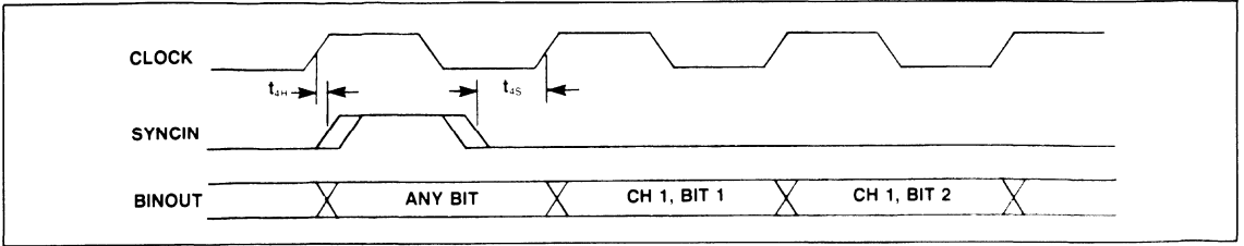
Figure 5. SYNCIN Timing Relationship
