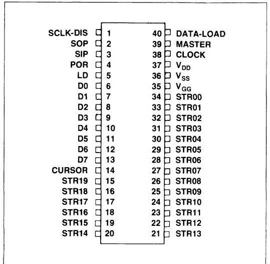
10939 Pin Configuration
