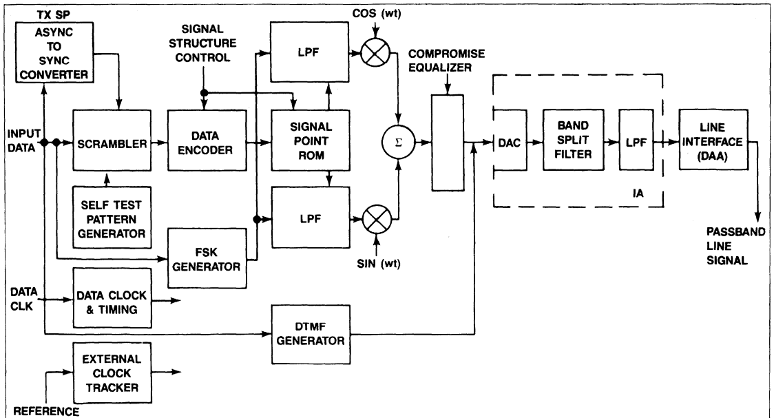
R1212 Transmitter Block Diagram
