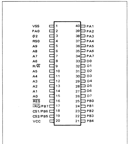
R6530 Pin Configuration
