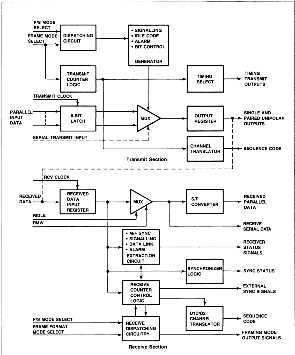
R8070 Functional Block Diagram
