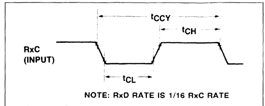
Figure 21. Receive External Clock Timing
