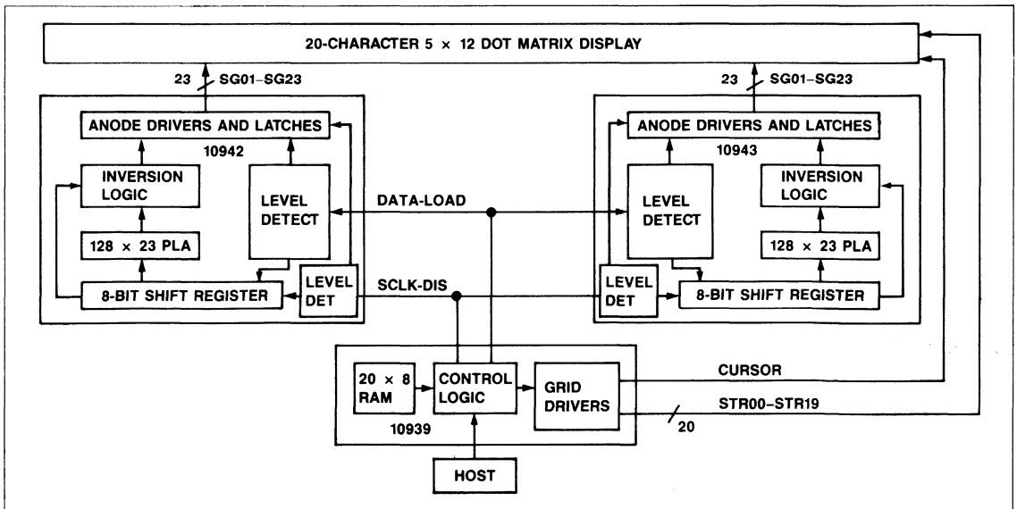
Block Diagram of 10939, 10942, 10943
