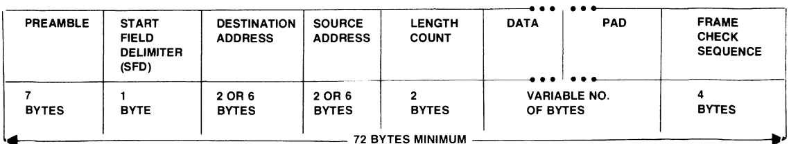
Figure 3. MAC Frame Format
