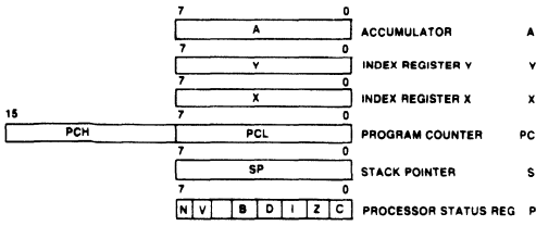
CPU Registers
