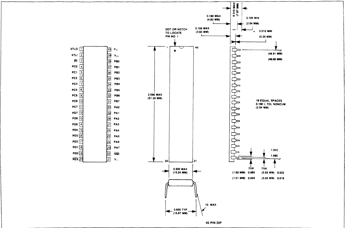
Figure 2-2. R6500/11 or /15 Mechanical Outline and Pin Out Configuration
