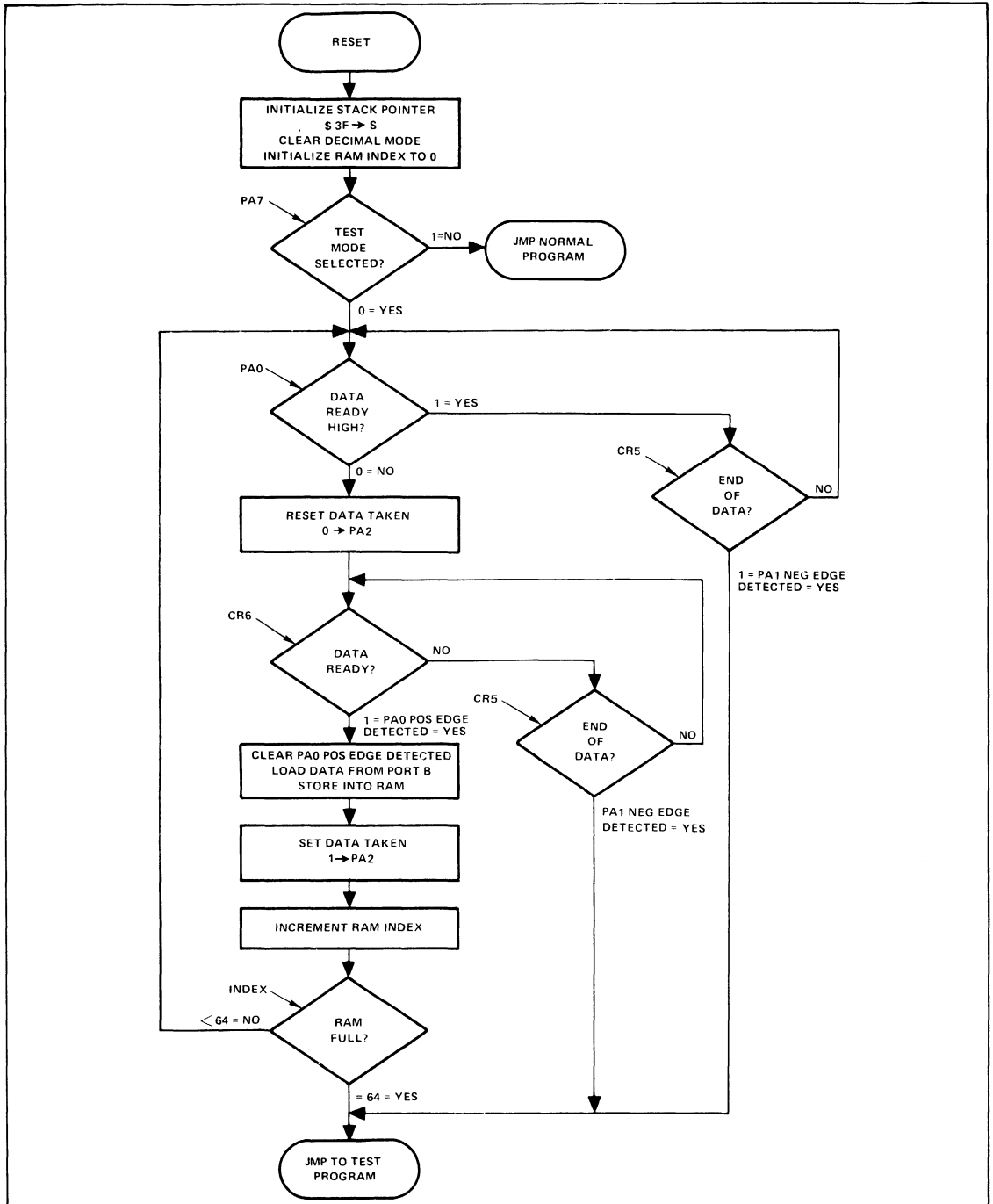
Figure 6-1. RAM Program Loader Flowchart
