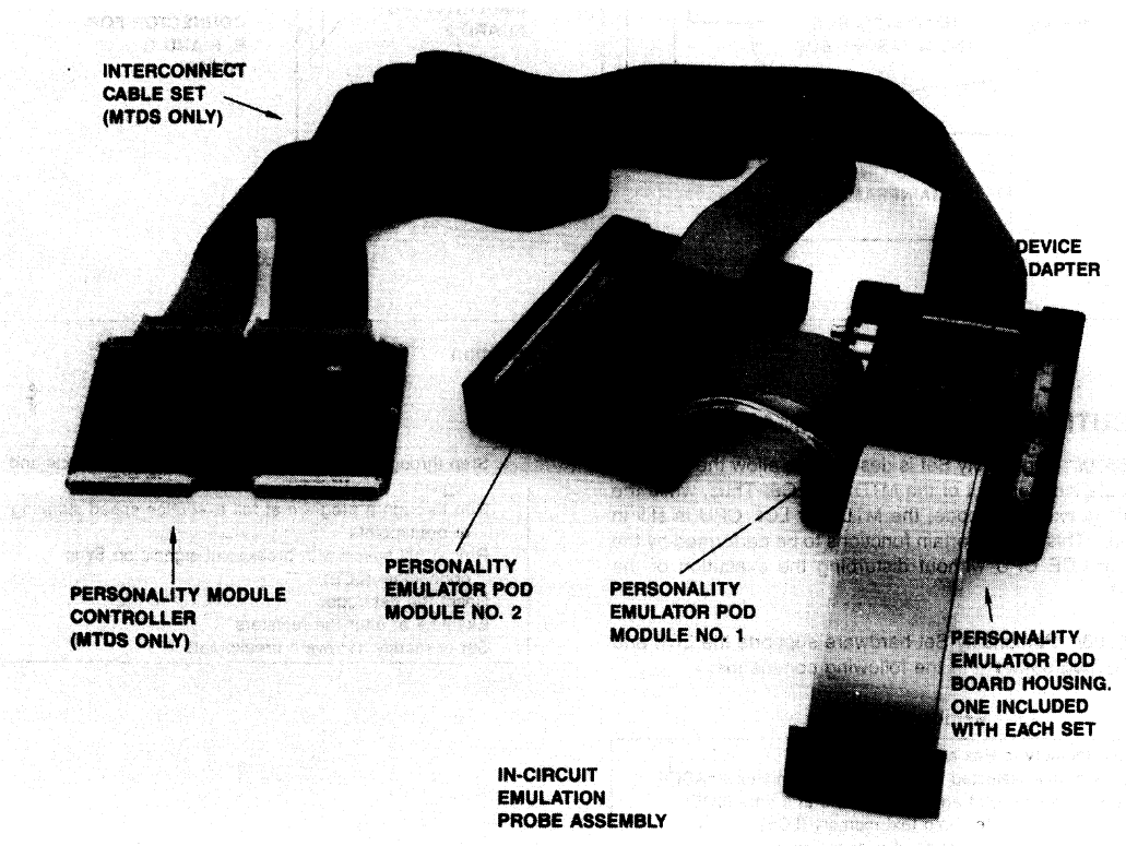
Typical R6500/* Personality Set Hardware Components
