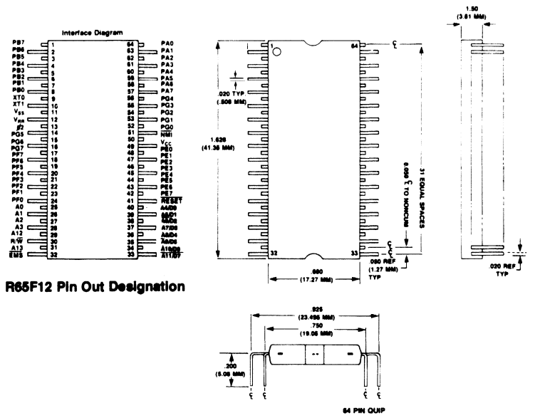
Figure 2-2. Pin Out Configuration
