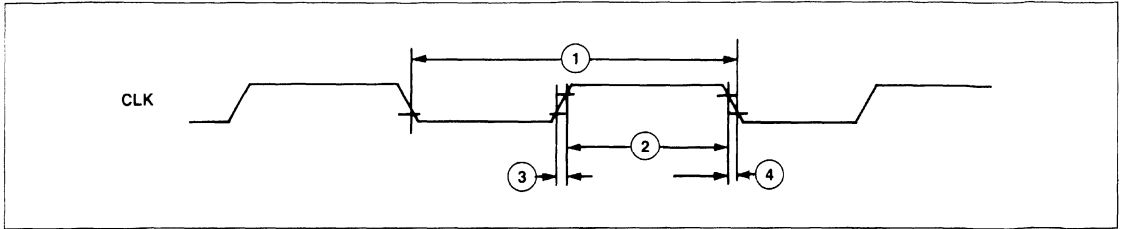
Figure 8. Clock Timing
