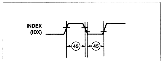
Figure 16. Index Timing
