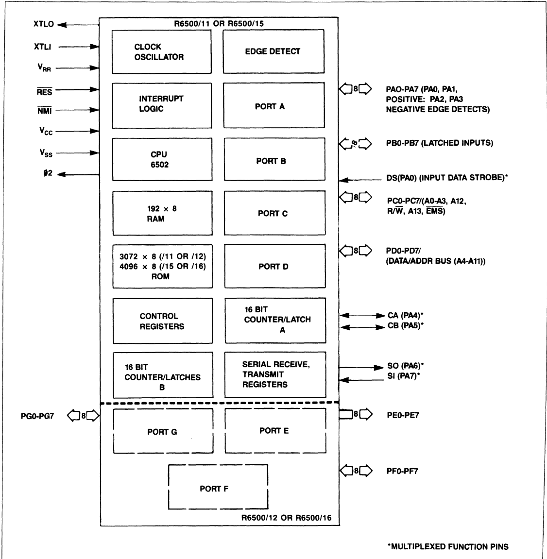
Figure 2.1 Interface Diagram
