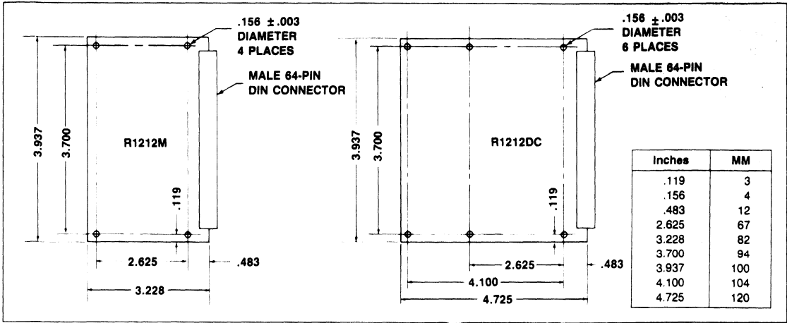
R1212 Printed Circuit Board Dimensions
