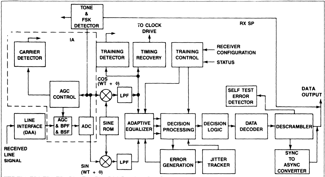
R1212/U Receiver/Equalizer Block Diagram
