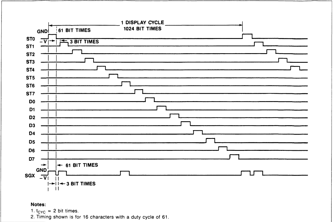
Display Scan Timing Diagram
