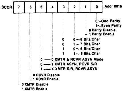
Serial Communications Control Register
