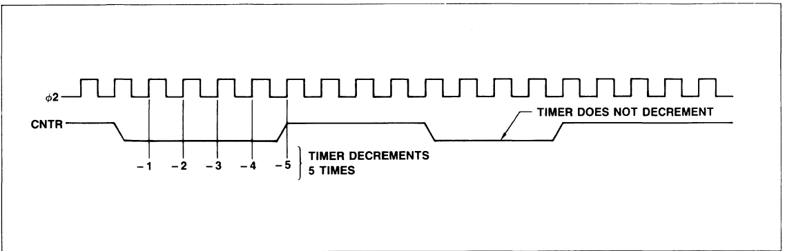
Figure 8. Mode 3—Pulse Width Measurement Timing
