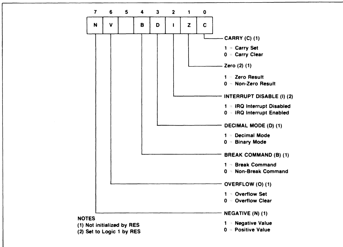
Figure 3-4. Processor Status Register
