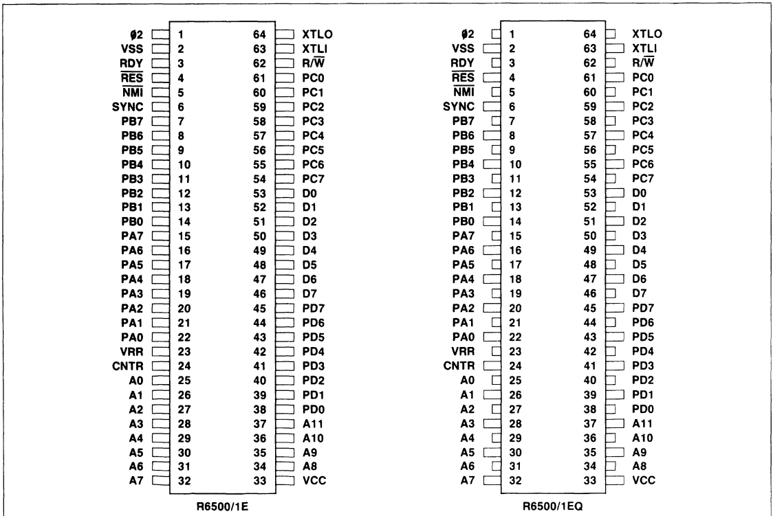
Pin Configuration
