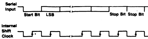
*Serial Input Data Shifted In
