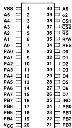
R6532 Pin Configuration
