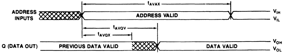
READ CYCLE TIMING 2
