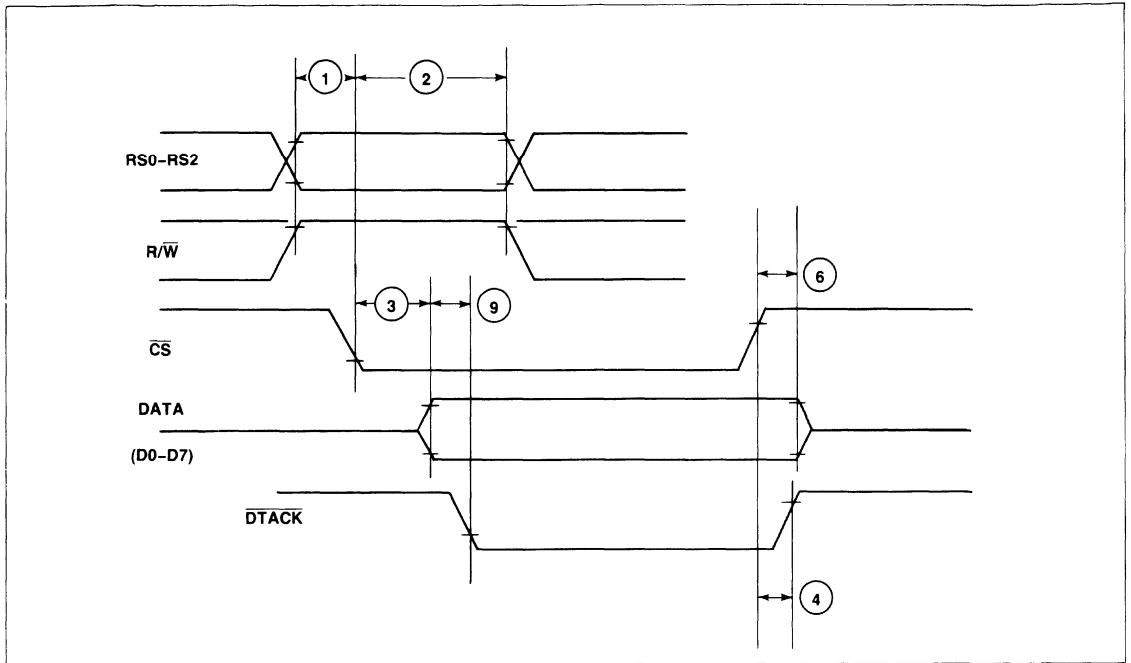
DACIA Read Cycle Timing
