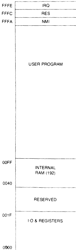
MEMORY MAP
