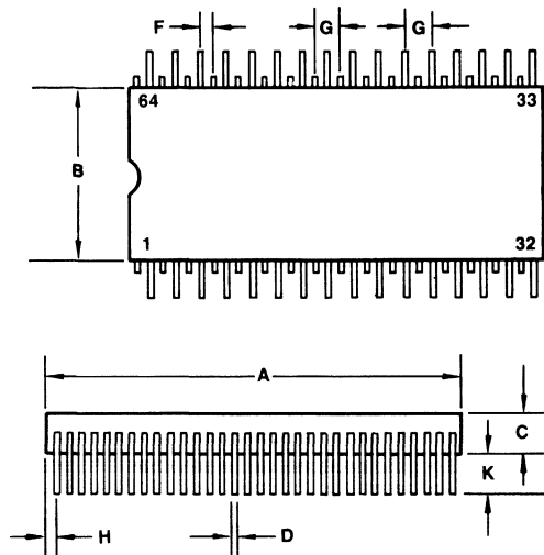
64 PIN PLASTIC QUIP (QUAD IN-LINE PACKAGE)
