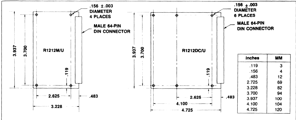
R1212/U Printed Circuit Board Dimensions
