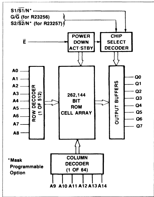
R23256 and R23257 Block Diagram
