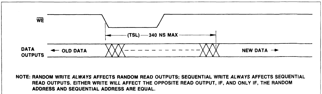
Read Outputs at Same Location as Write (All Other Inputs Stable)
