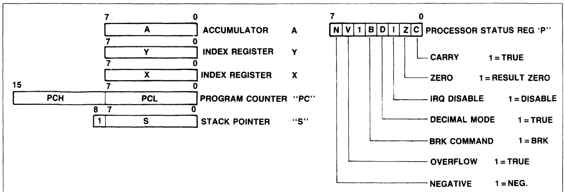
Programming Model
