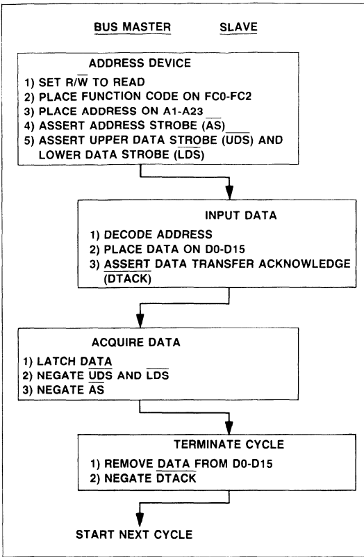
Figure 4. Word Read Cycle Flow Chart
