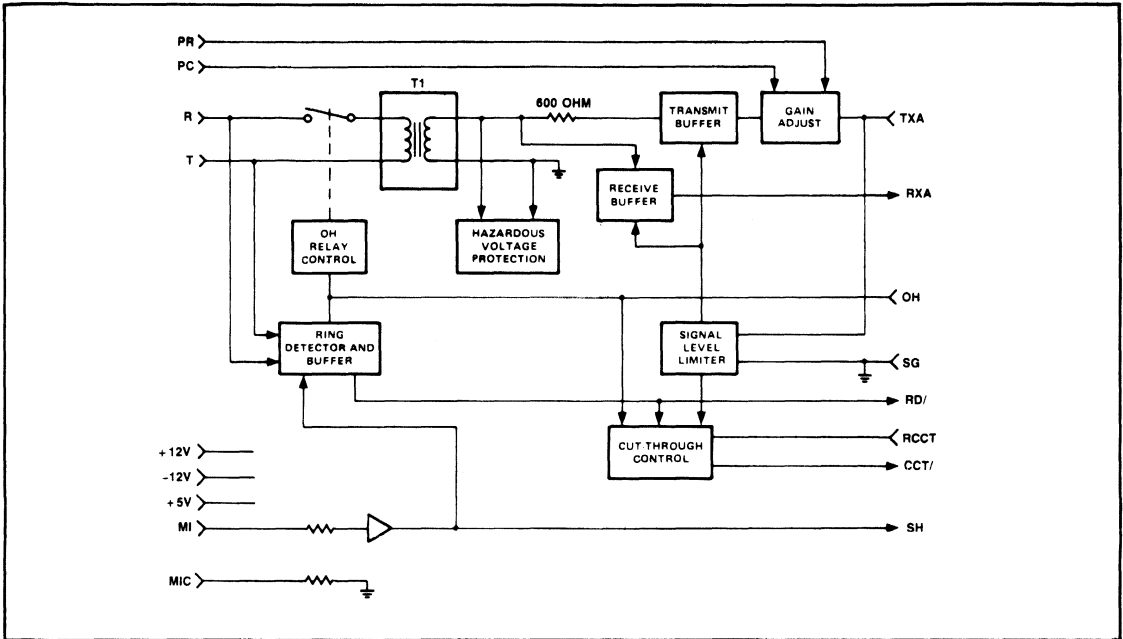
Figure 3. RDA Functional Block Diagram
