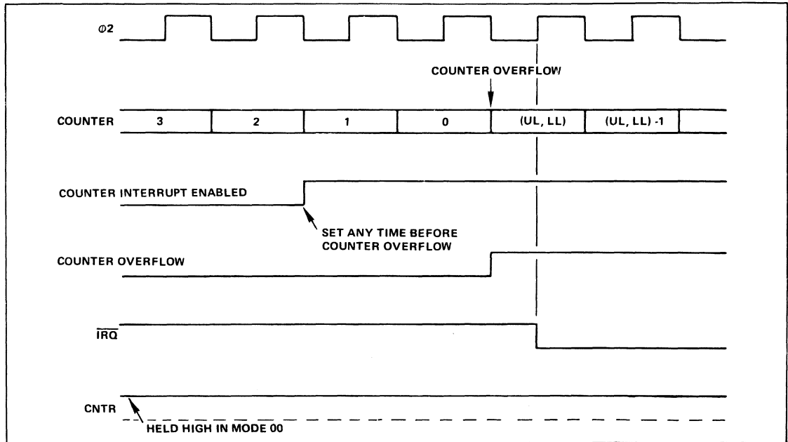
Figure 3-5. Interval Timer (Mode 0) Timing Diagram
