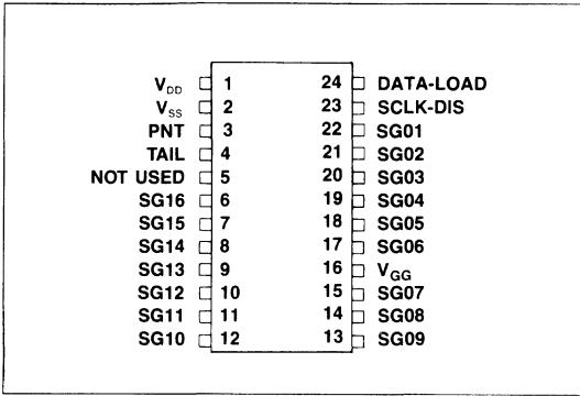
10941 Pin Configuration
