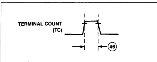
Figure 17. Terminal Count Timing
