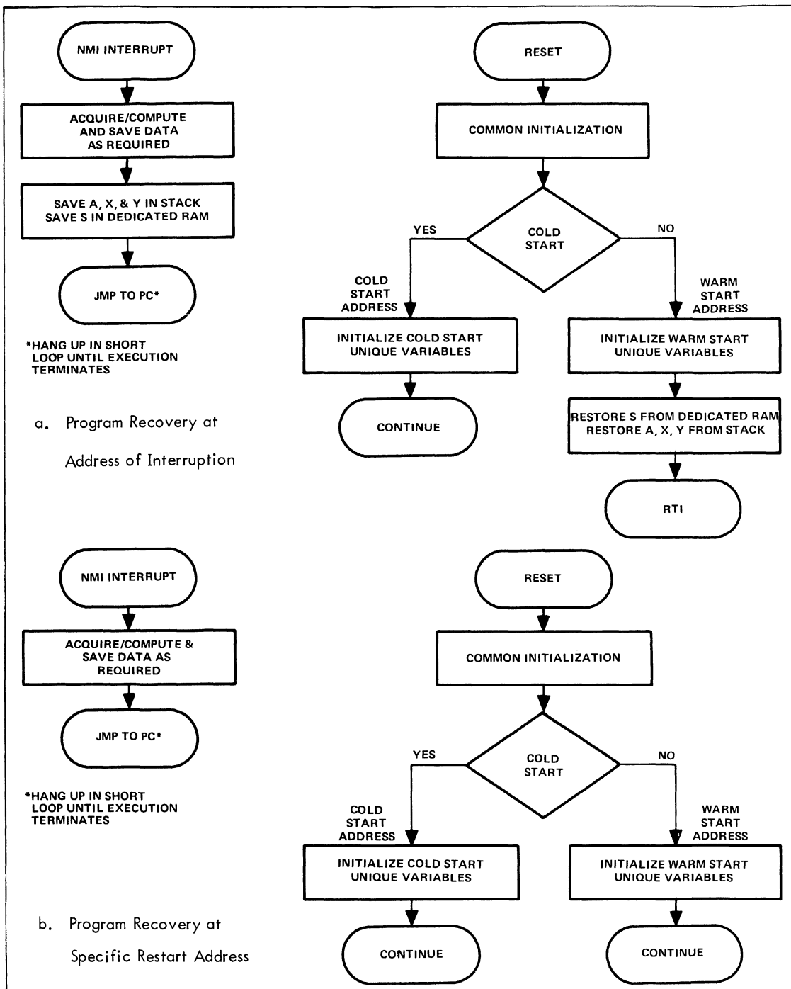
Figure 5-3. Typical R6500/1 Power Loss Recovery Flowcharts
