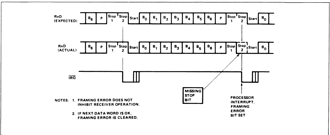
Figure 13. Framing Error
