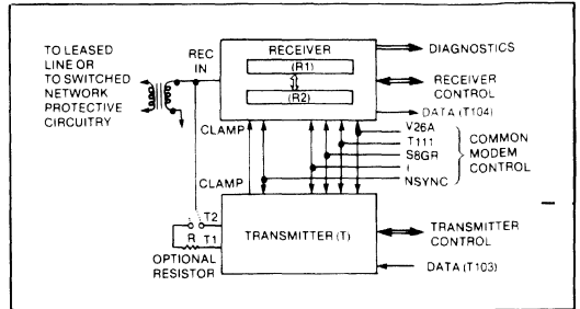
Figure 3. Transmitter-Receiver Interconnection (Half Duplex)
