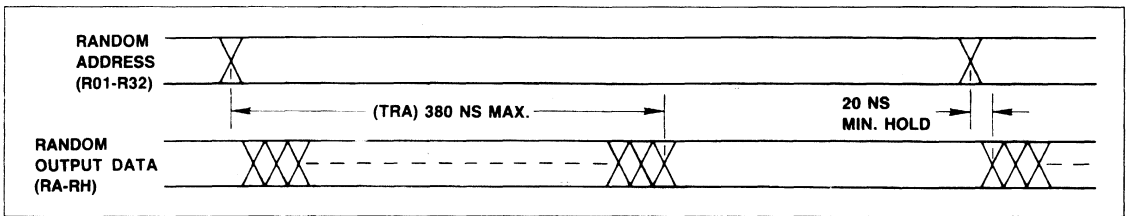
Random Read ( \overline{RRE} = 0, \overline{WE} = 1 )
