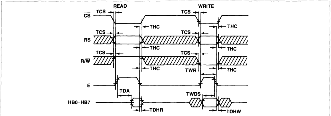
Figure 5-3. Timing Diagram—Host Interface (MCR4 = 0) (6500 Version)
