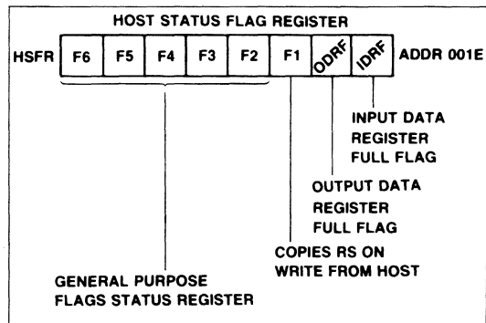
Figure 5-1. Host Status Flag Register Bit Allocation
