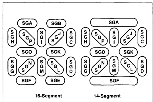
Figure 1. Segment Driver Assignments
