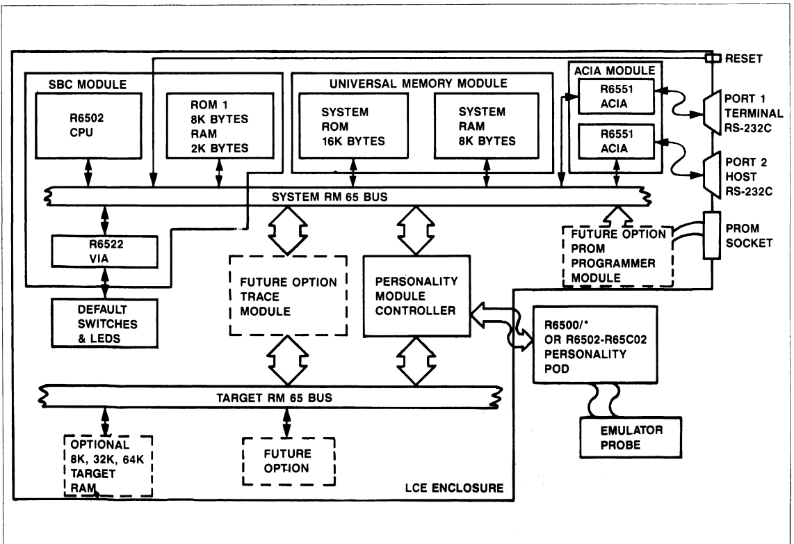
LCE System Block Diagram
