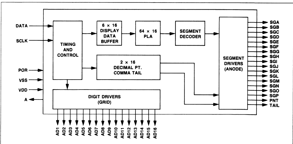
10951 Block Diagram
