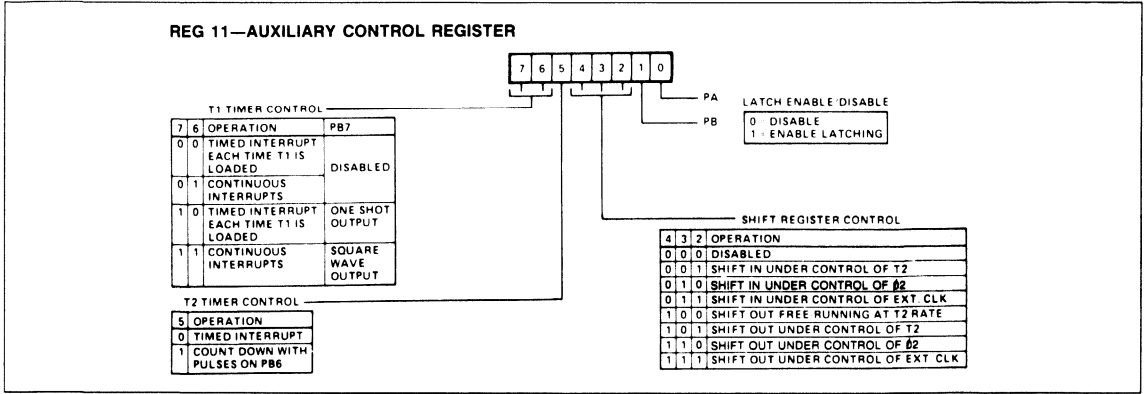
Figure 14. Auxilliary Control Register (ACR)
