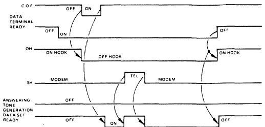
Automatic Call Mode Sequence
