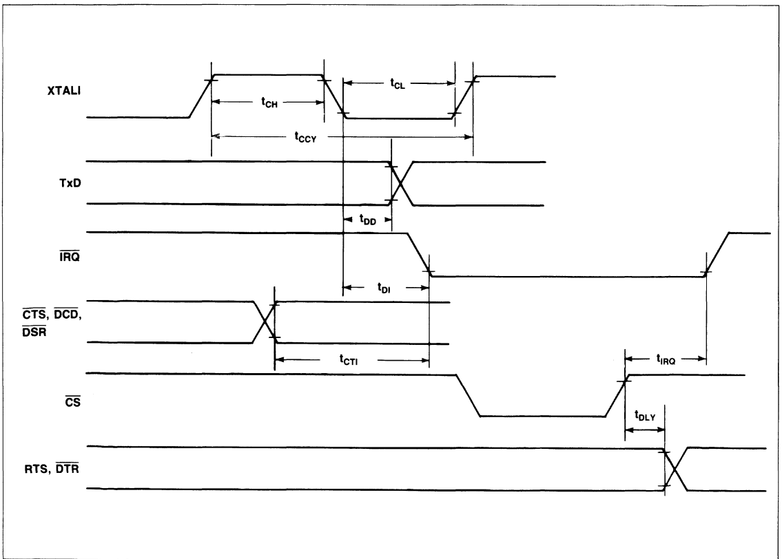
DACIA Transmit/Receive Timing
