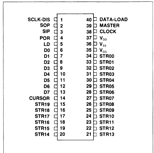
10939 Pin Configuration
