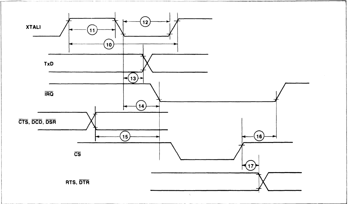
DACIA Transmt/Receiver Timing
