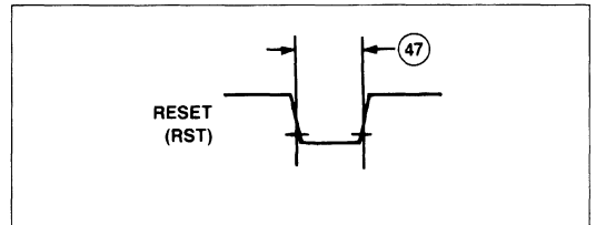
Figure 18. Reset Timing
