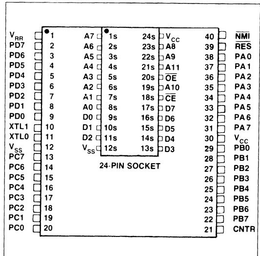
Pin Configuration
