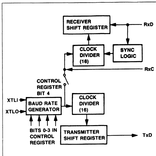
Figure 3. Transmitter/Receiver Clock Circuits
