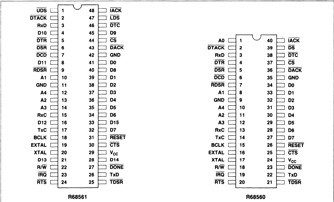
Pin Configuration
