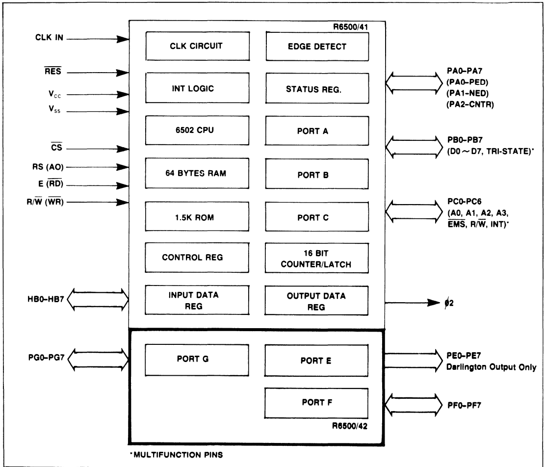
Figure 2-1. Interface Diagram
