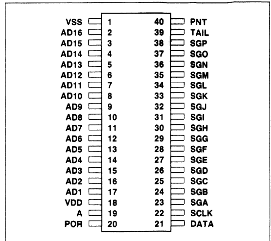
10951 Pin Configuration
