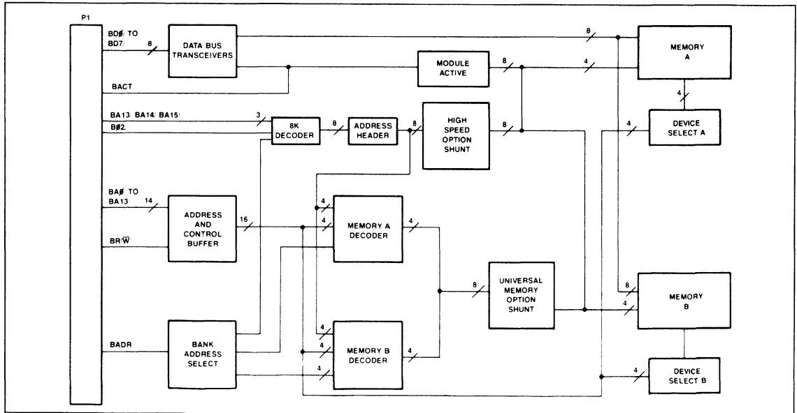
Target RAM Module Block Diagram
