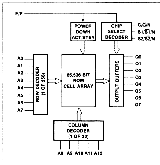
R2364B Block Diagram
