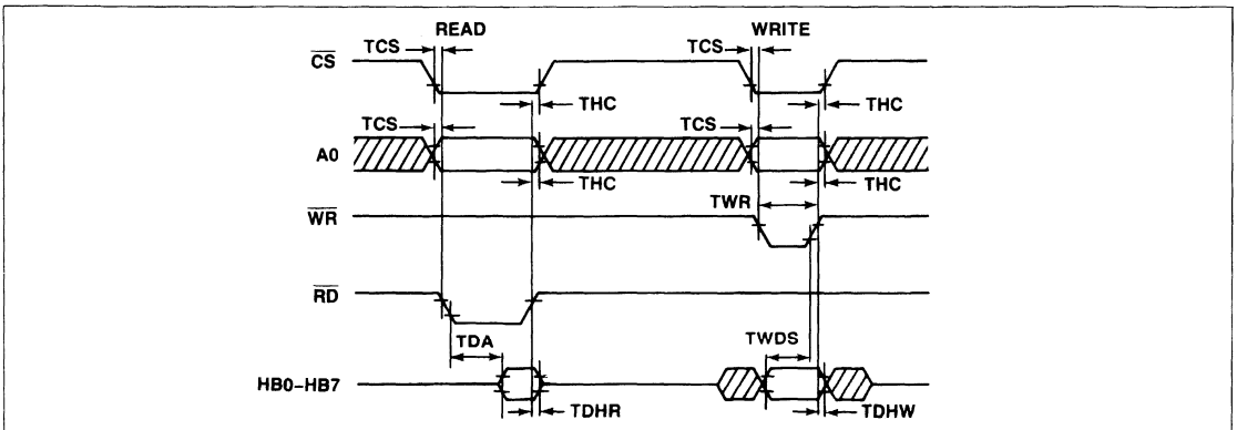
Figure 5-4. Timing Diagram—Host Interface (MCR4 = 1) (8080 Version)
