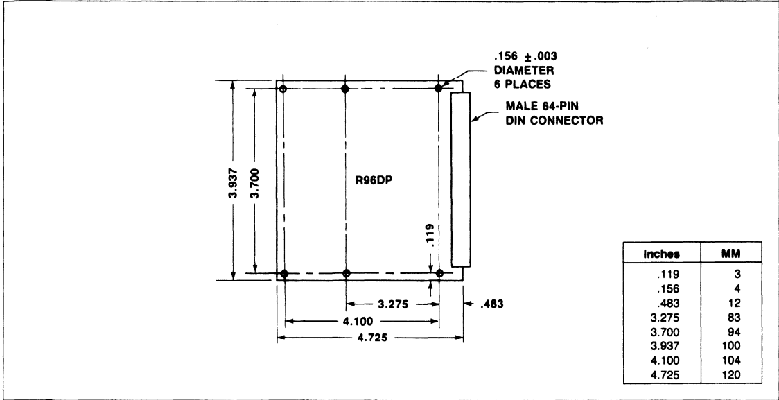
R96DP Circuit Board Dimensions
